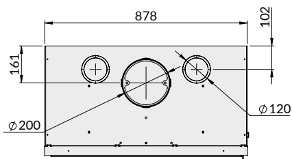
Vista topo Vista superior Top view
