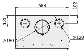
Vista topo Vista superior Top view
