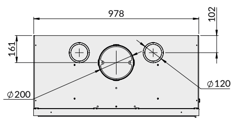
Vista topo Vista superior Top view
