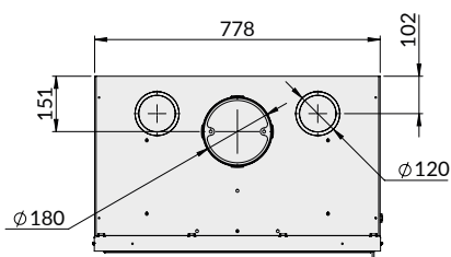
Vista topo Vista superior Top view
